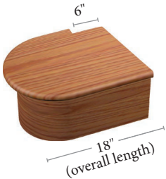
8010-2 False End and Riser - 12½" x 18" 8310-2 False End and Riser - 14" x 18"
